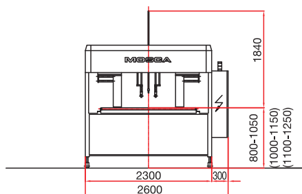
Technical drawing corresponds to UATRI 1300
